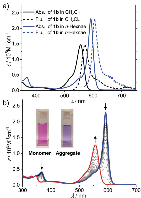
Fig. 1 (a) UV/Vis absorption and fluorescence spectra ( \lambda_{\text{Ex}} = 350 nm) of dye 1b in CH 2 Cl 2 (black, c T = 2.0 × 10 −6 M) and n -hexane (blue, c T = 2.0 × 10 −6 M). (b) Temperature-dependent UV/Vis absorption spectra of BODIPY dye 1b in n -hexane ( c T = 2.0 × 10 −6 M). The arrows indicate the spectra changing with the increase of the temperature from 277 to 333 K. Inset: Visual appearance of solutions of monomeric and aggregated dye 1b under daylight.
