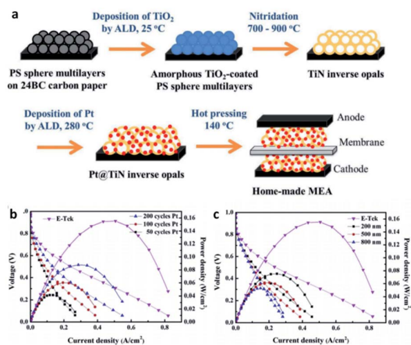
Fig. 8 (a) Schematic of fabricating Pt@TiN@CP to form MEA for PEMFCs. MEA performances for home-made anodes with (b) Pt prepared by various cycle numbers of ALD on 500 nm TiN inverse opals and (c) Pt prepared by 100 ALD cycles on TiN inverse opals with different diameters. The commercial E-Tek anode is included for comparison. For all cases, E-Tek electrode is used as the cathode. Reproduced with permission from ref. 110. Copyright © 2017 Elsevier Ltd.
