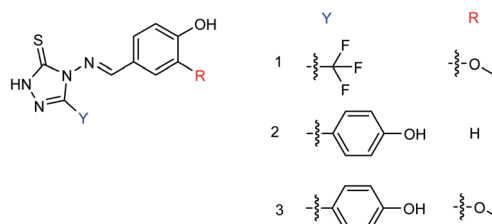
Fig. 49 Structure of 4-(arylimino)-3-alkyl-1H-1,2,4-triazol-5(4H)-thio ketone derivatives.
