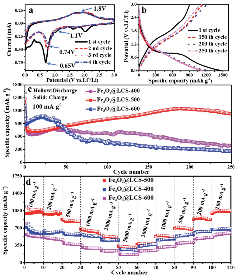
Fig. 3 Lithium storage performances of \text{Fe}_3\text{O}_4@LCS-(400/500/600) electrodes: (a) CV curves in the first four cycles at a scan rate of 0.1 \text{ mV s}^{-1} ; (b) charge/discharge profiles at 100 \text{ mA g}^{-1} ; (c) cycle performances of \text{Fe}_3\text{O}_4@LCS-(400/500/600) at the current density of 100 \text{ mA g}^{-1} for 250 cycles; (d) the rate performance of \text{Fe}_3\text{O}_4@LCS-(400/500/600) at various current densities.
