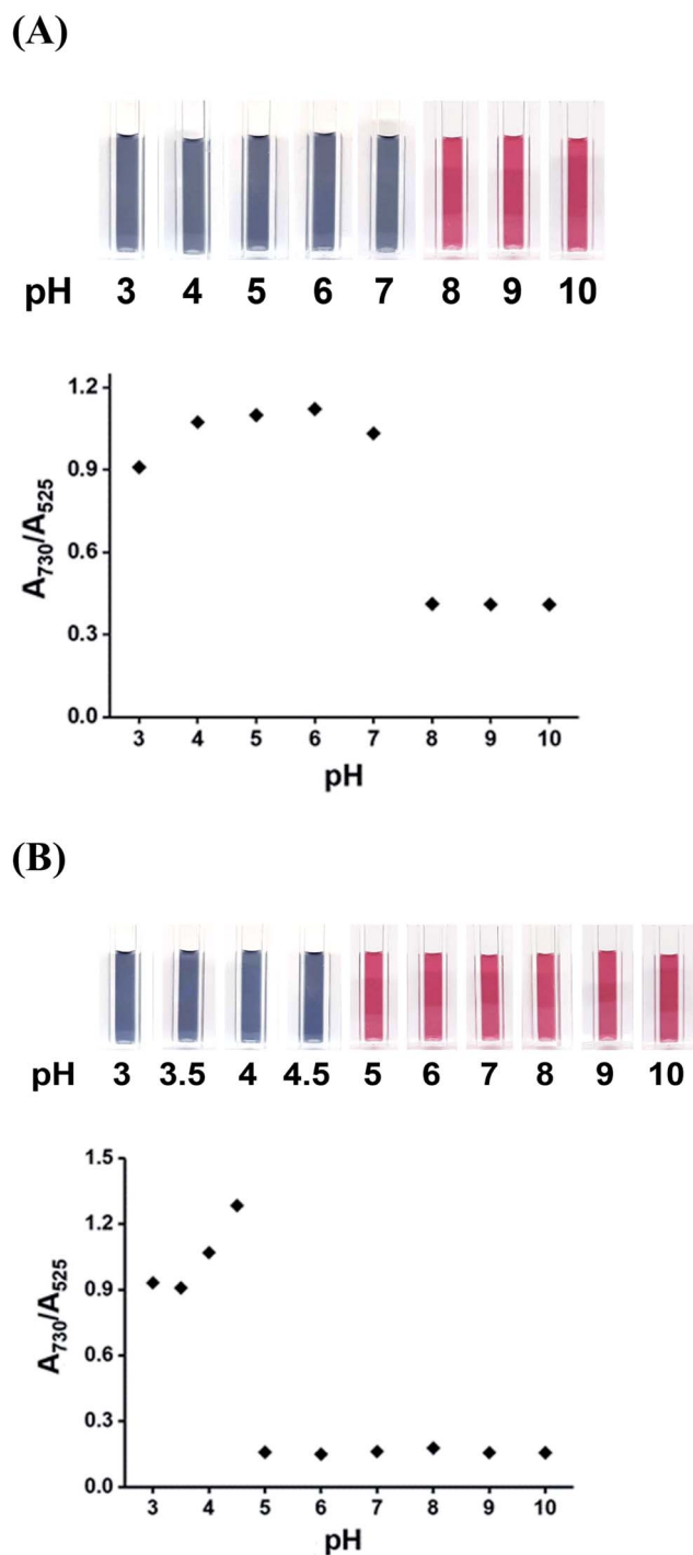
Fig. 6 Photographic images and absorption ratios ( A_{730}/A_{525} ) of DPL-AuNP in the presence of (A) 5.0 \mu\text{M} \text{Hg}^{2+} ions, and (B) 5.0 \mu\text{M} \text{As}^{3+} ions as a function of pH.
