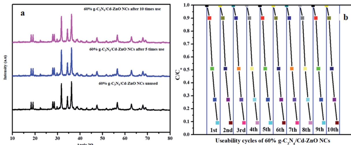
Fig. 12 (a) XRD patterns of the 60% g-C 3 N 4 /Cd-ZnO NCs before use, after 5-times use after 10-time uses, and (b) 10 usability cycles for the 60% g-C 3 N 4 /Cd-ZnO NCs.
