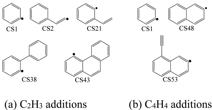
Fig. 15 Aromatic structures for C_2H_3 and C_4H_4 additions.
