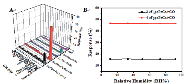
Fig. 3 (A) Response of RPCos, rGO and RPOCo/rGO hybrid-based sensors to 1 ppm of H 2 S and 1000 ppm of various other gases, respectively. (B) Response of the cF 3 poPcCo/rGO hybrid-based sensors to 1 ppm H 2 S at different relative humidities at 25 °C.
