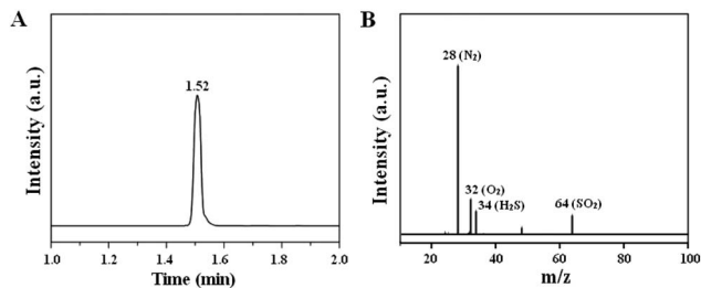
Fig. 5 (A) Gas chromatogram and (B) mass spectrum after 4- \text{cF}_3 - \text{poPcCo/rGO} sensor exposure to \text{H}_2\text{S} at 25 °C.
