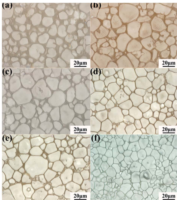
Fig. 2 Surface morphologies of \text{BCZT}_x\text{C}_y\text{S}_z ceramics: (a) BCZT; (b) x = 0.10 ; (c) y = 0.10 ; (d) x = 0.05 , y = 0.10 ; (e) x = 0.10 , y = 0.10 ; (f) x = 0.15 , y = 0.10 .
