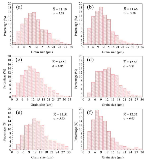
Fig. 3 Grain size distribution in \text{BCZT}_x\text{C}_y\text{S}_z ceramics: (a) BCZT; (b) x = 0.10 ; (c) y = 0.10 ; (d) x = 0.05 , y = 0.10 ; (e) x = 0.10 , y = 0.10 ; (f) x = 0.15 , y = 0.10 .
