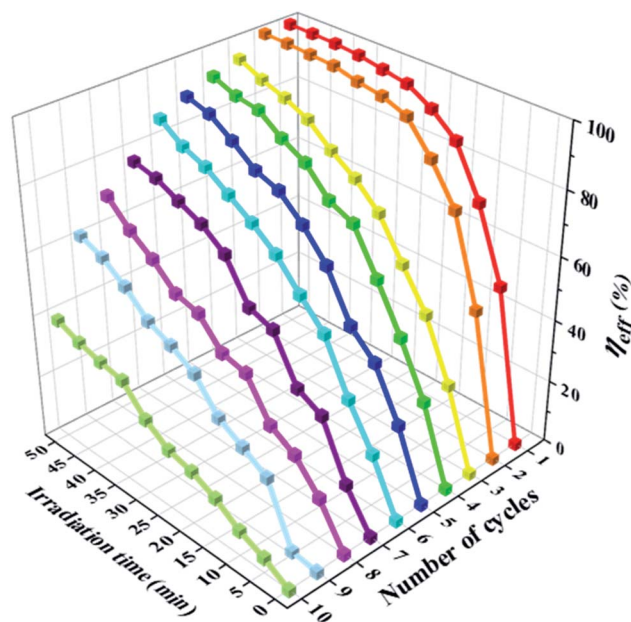
Fig. 8 Photodegradation rates curves for ENR ( 10 \text{ mg} \cdot \text{L}^{-1} ) aqueous solution using Ag-ZnFe_2O_4 -rGO photocatalysts for 10 cycles under visible-light irradiation.
