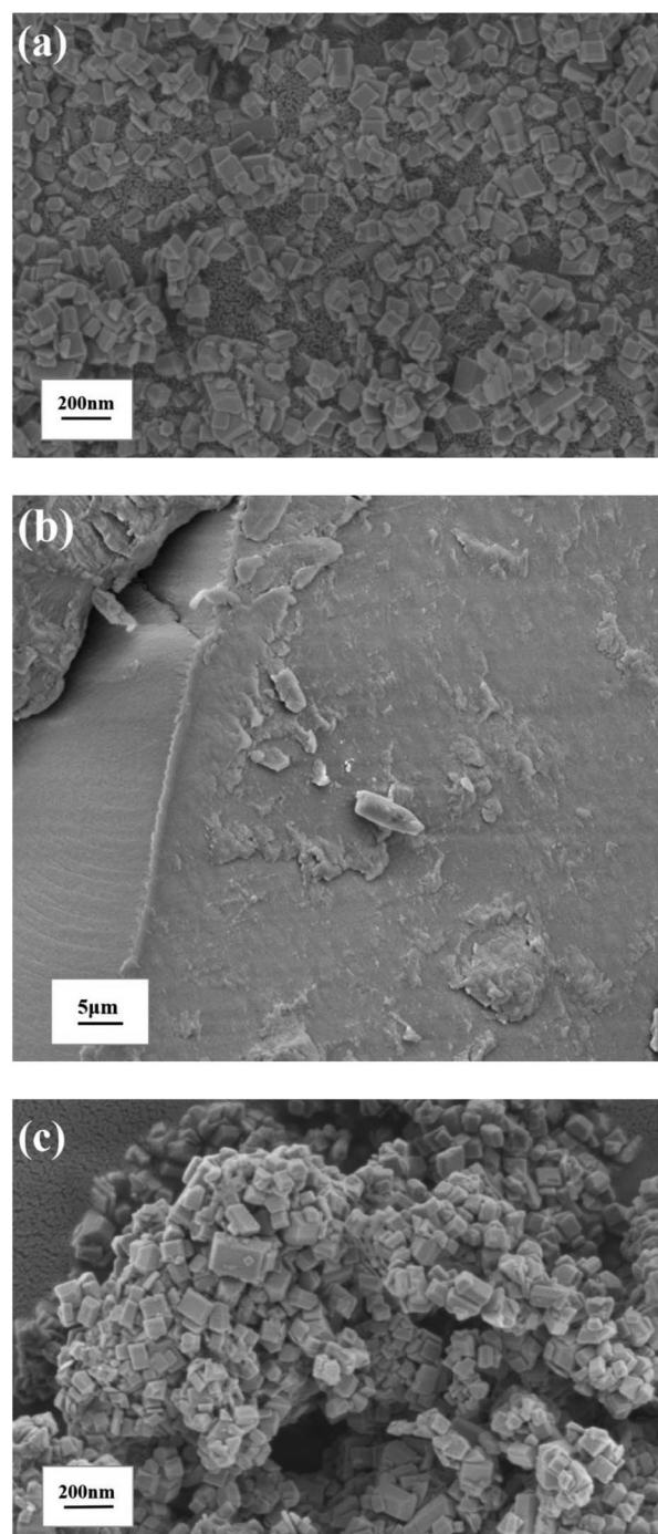
Fig. 1 Scanning electron microscopy images of (a) \text{TiO}_2\text{-}_x\text{F}_x , (b) CTFs and (c) \text{TiO}_2\text{-}_x\text{F}_x /CTFs.
