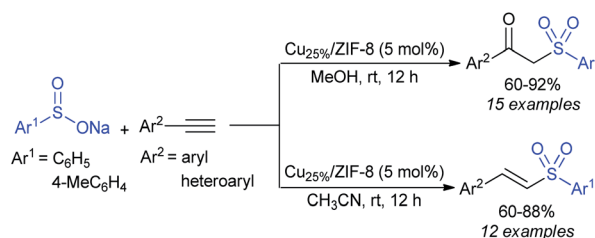
Scheme 133 \text{Cu}_{25\%}/\text{ZIF-8} -catalyzed oxy-sulfonation and hydro-sulfonation of terminal alkynes with sodium sulfonates.
