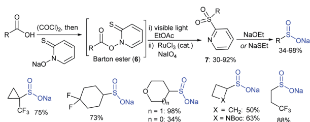
Scheme 7 Synthesis of new types of sodium sulfinates.
