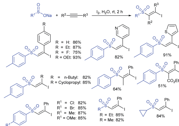
Scheme 124 I 2 -mediated iodosulfonylation of alkynes using sodium sulfonates.
