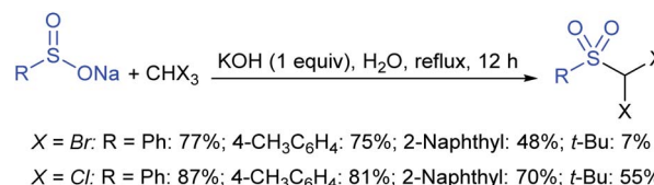
Scheme 251 KOH-mediated coupling of sodium sulfonates with haloforms.
