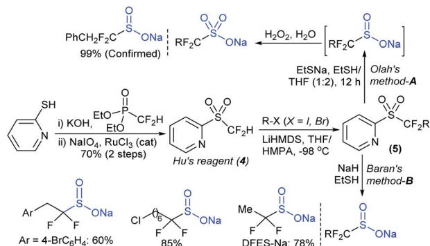
Scheme 6 Preparation of alkyl \alpha,\alpha -difluoro sodium sulfinates.
