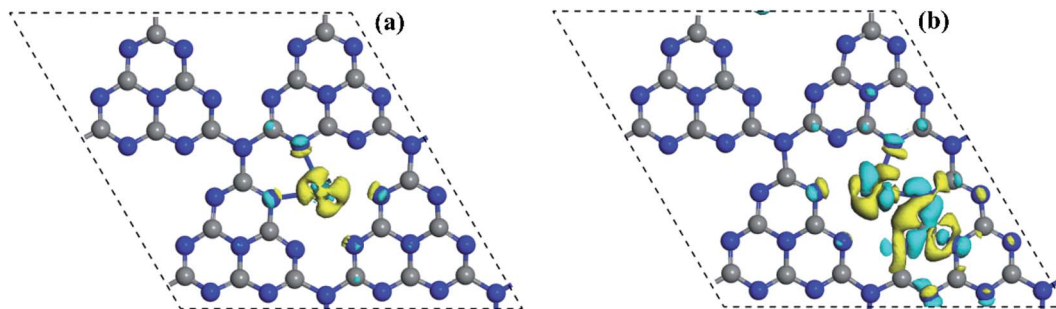
Fig. 7 Plots of 3D charge density difference of (a) \text{Pd}_1\text{@g-C}_3\text{N}_4 and (b) \text{Pt}_1\text{@g-C}_3\text{N}_4 at isosurfaces of \pm 0.05 \text{ e } \text{\AA}^{-3} . The blue and yellow colours represent charge accumulation and depletion, respectively. The balls in gray and blue represent the C and N atoms, respectively.
