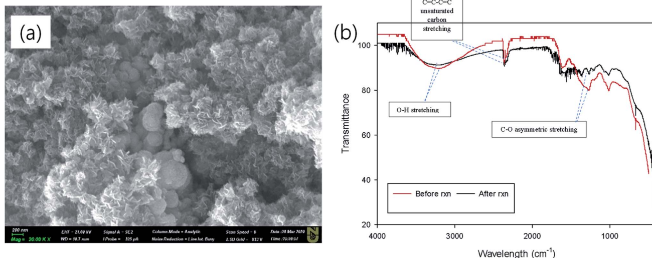
Fig. 7 SEM image (a) and FTIR spectra (b) of G-NZVI after BrO 3 - reduction.
