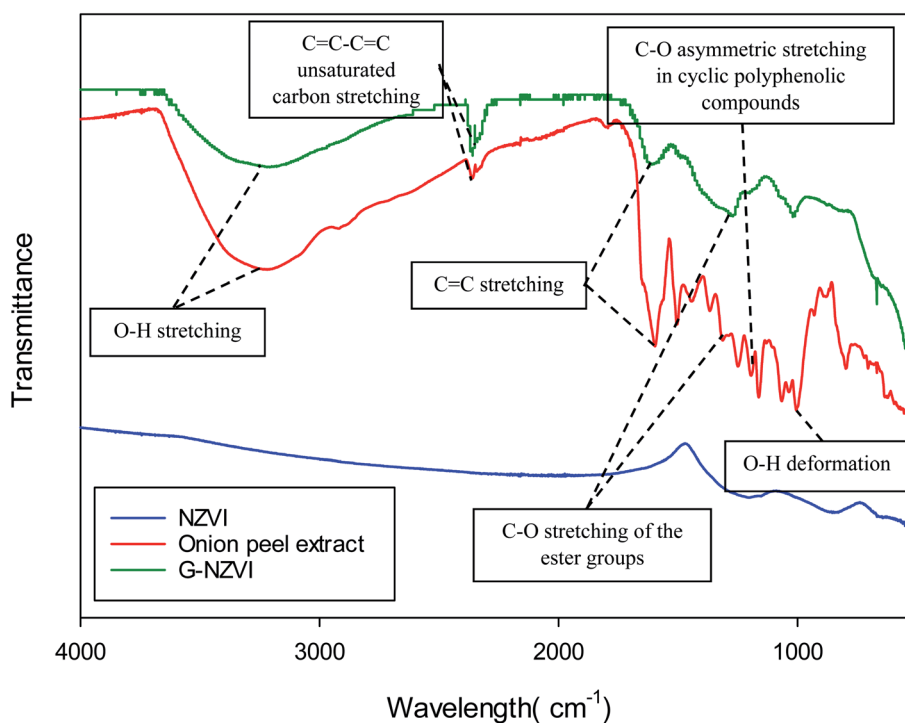
Fig. 3 The FTIR spectra of the onion peel extract, NZVI, and G-NZVI.
