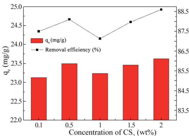
Fig. 2 \text{La}(\text{III}) adsorbed by functionalized \text{MWCNT}@Fe_3O_4 with variable \text{CS}_2 concentrations, [\text{ECH}] = 0.1 \text{ wt}\% .
