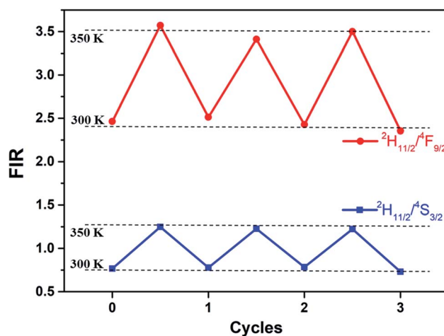
Fig. 7 FIR of Er 3+ 2 H 11/2 / 4 S 3/2 and 2 H 11/2 / 4 F 9/2 at 300 and 350 K in three cycles of heating and cooling for the core-shell UCNPs (the dots are experimental data).
