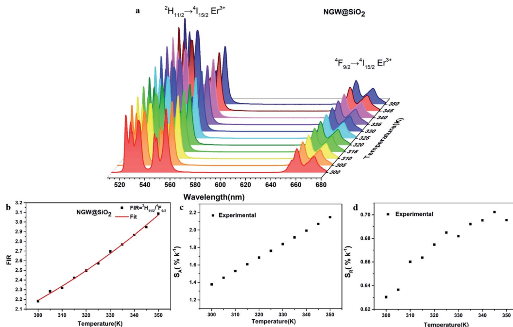
Fig. 6 FIR analysis of the 2 H 11/2 green emission to the red 4 F 9/2 emission for the core-shell NGW:Yb 3+ /Er 3+ @SiO 2 UCNPs in the temperature range from 300 K to 350 K. (a) UC emission spectra under 980 nm laser excitation (power density of 162 mW cm -2 ). The spectra are normalized to the emission peak at 657 nm. (b) FIR, (c) S A , and (d) S R versus temperature.
