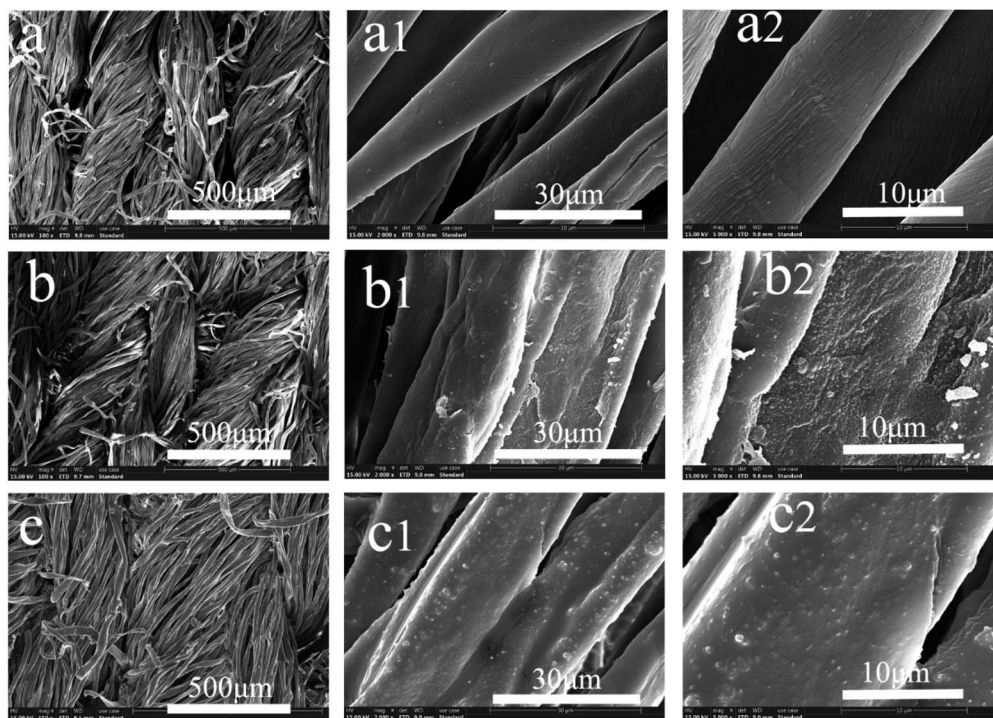
Fig. 3 SEM images of pristine cotton (a), SiO 2 -SH@cotton (b) and SiO 2 -S-PIH@cotton (c) at 100, 2000, and 5000 SE, respectively.
