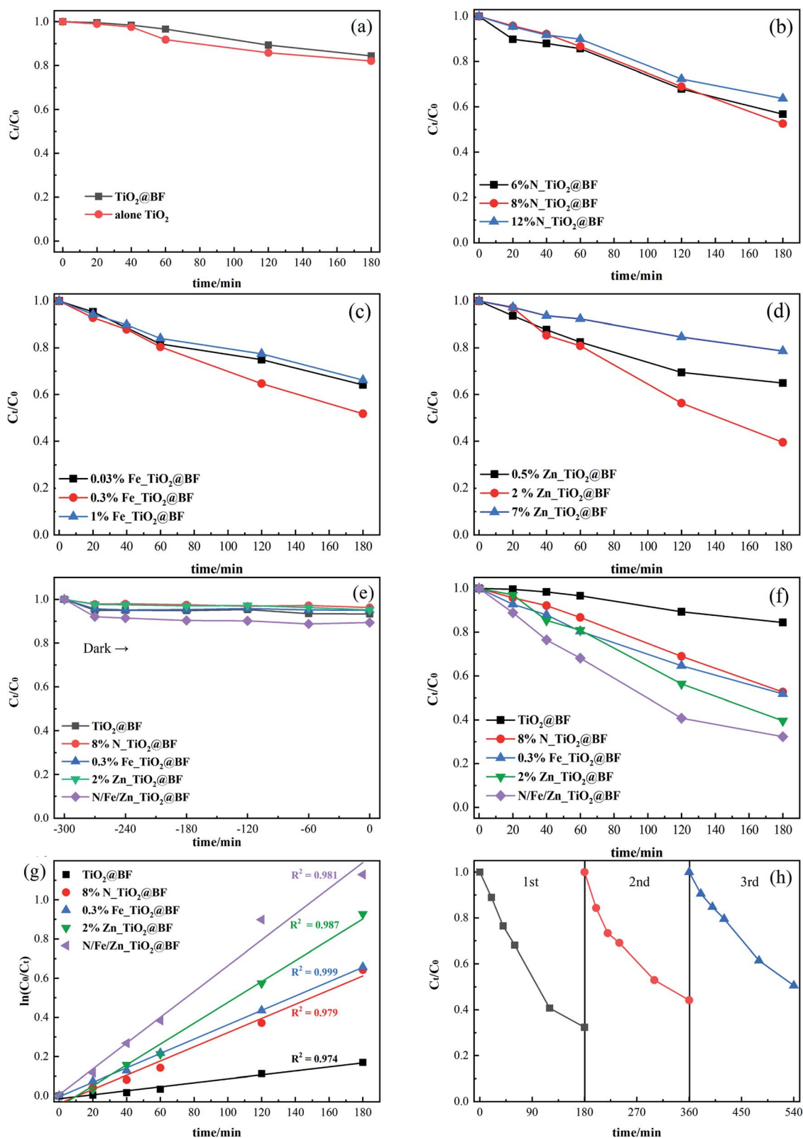
Fig. 7 (a) Photocatalytic activity of the same amount of \text{TiO}_2 without loading on BF and \text{TiO}_2@\text{BF} , (b–d, f) photocatalytic activities (in the degradation of RhB) of \text{TiO}_2@\text{BF} and \text{G}_\text{N}-\text{TiO}_2@\text{BF} doped with different substances at different doping ratios, (e) dark adsorption curves, (g) photocatalytic degradation kinetics and (h) the stability and reusability tests of N/Fe/Zn- \text{TiO}_2@\text{BF} for RhB removal.
