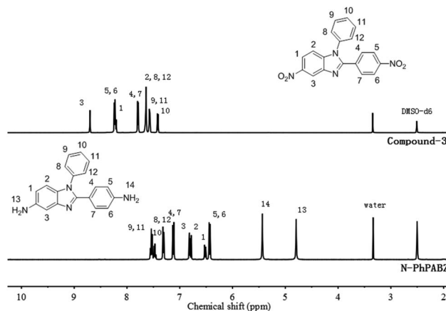
Fig. 1 1 H NMR spectra of synthesized monomers (compound 3 and N -PhPABZ).
