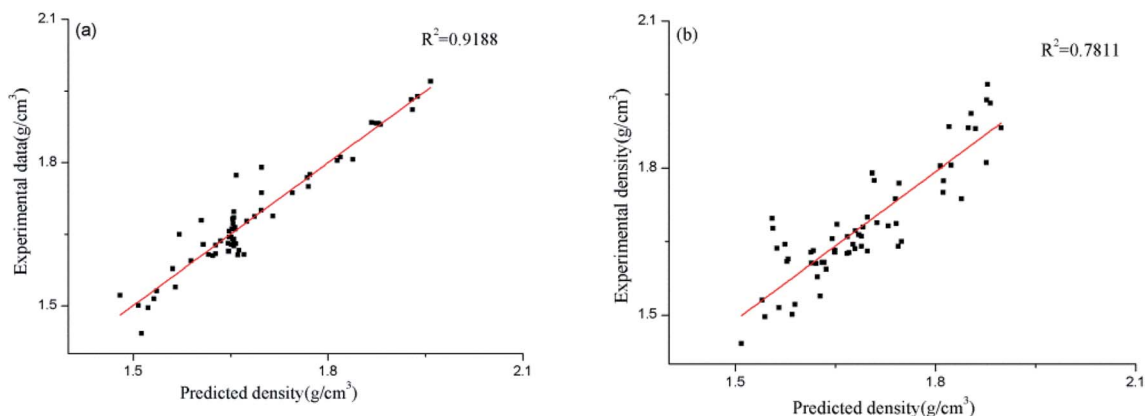
Fig. 2 Predicted densities of the cococrystals vs. experimental data for all the datasets ((a) for the ANN model, and (b) for the Politzer model).
