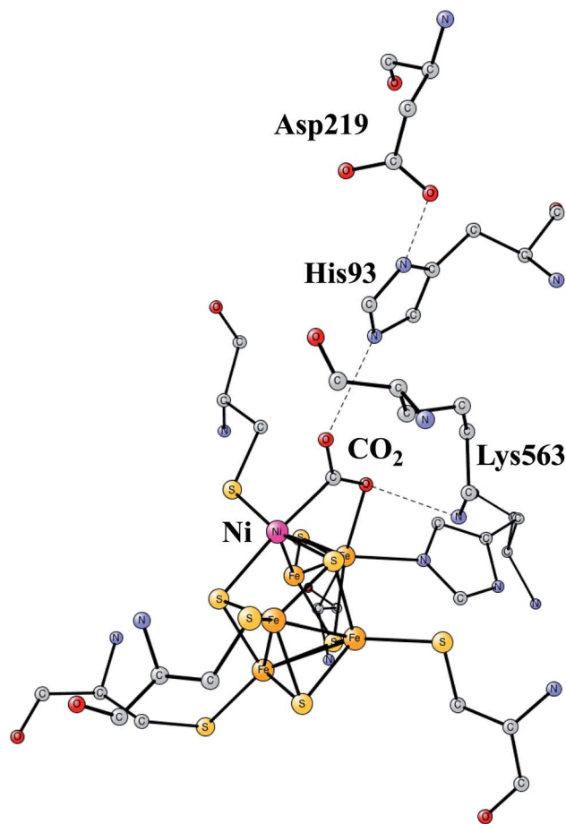
Fig. 13 The X-ray structure of the active site for NiFe-CODH, showing the key intermediate with a bound CO 2 . 61
