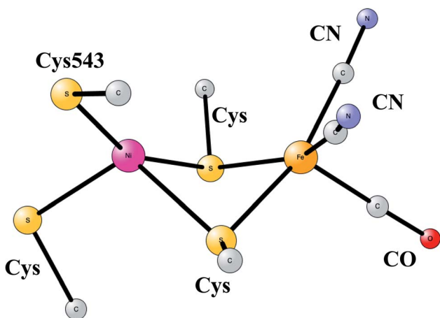
Fig. 10 Optimized structure for the active site of NiFe hydrogenase, based on an X-ray-structure. 44,45
