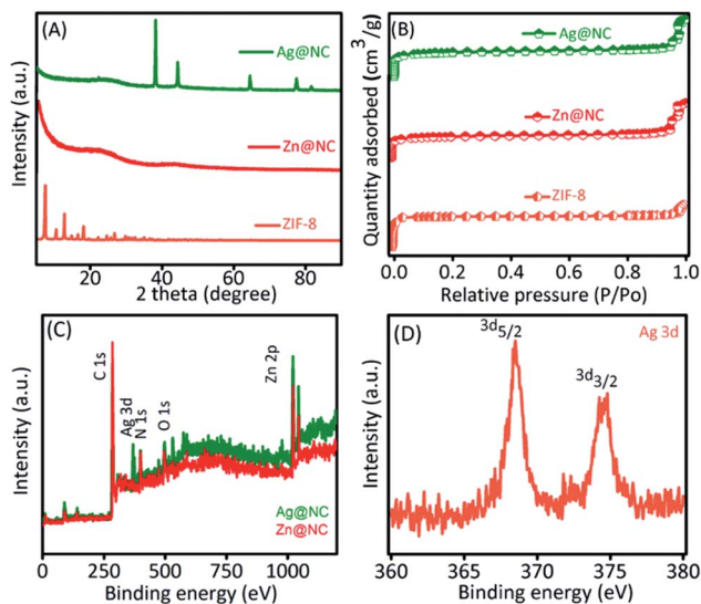
Fig. 2 (A) XRD pattern and (B) N 2 adsorption/desorption analysis of the ZIF-8, the Zn@NC and the Ag@NC samples. (C) XPS survey spectra of the Ag@NC sample and (D) the chemical state of Ag.
