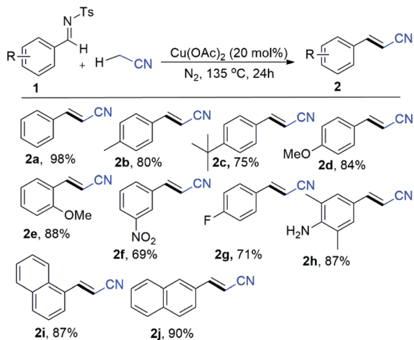
Scheme 3 Substrate scope for imines using \text{CH}_3\text{CN} . a,b a Conditions: 1 (0.2 mmol), \text{Cu}(\text{OAc})_2 (20 mol%), \text{N}_2 , 135\text{ }^\circ\text{C} , \text{CH}_3\text{CN} (1.2 mL), 24 h. b Isolated yield.
