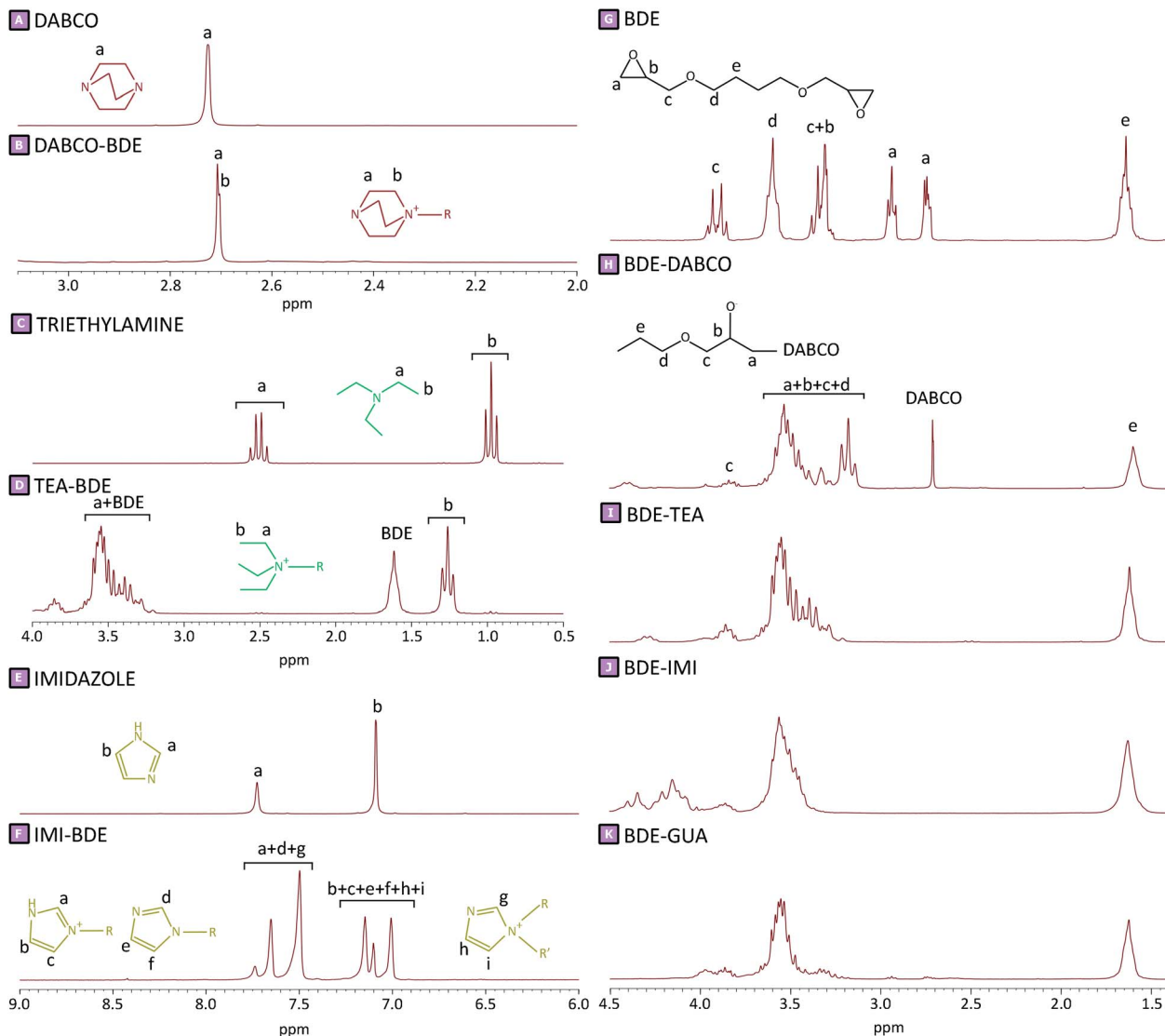
Fig. 6 1 H NMR spectra of DABCO, TEA, and IMI before and after reaction with BDE (A–F). 1 H NMR spectra of BDE before and after reaction with DABCO, TEA, IMI, and GUA (G–K).
