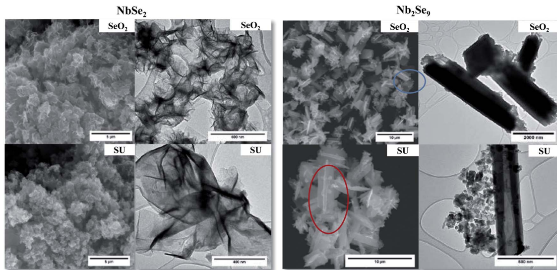
Fig. 12 SEM and TEM images of \text{NbSe}_2 and \text{Nb}_2\text{Se}_9 when varying the selenium precursors.
