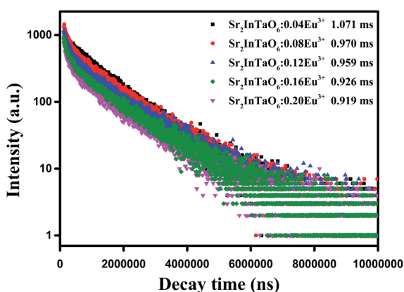
Fig. 7 The decay curves and calculated lifetimes of \text{Sr}_2\text{InTaO}_6:\text{xEu}^{3+} samples under 394 nm excitation and monitored at 624 nm.
