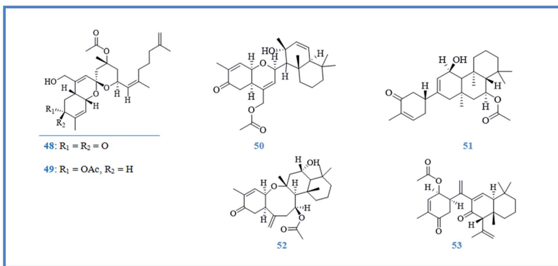
Fig. 9 Structure of compounds 48–53.
