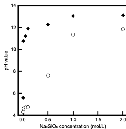
Fig. 1 The initial ( \blacklozenge ) and final ( \circ ) pH values, respectively, of the reaction solutions with different \text{Na}_2\text{SiO}_3 concentrations.
