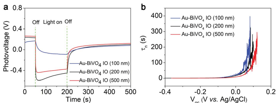
Fig. 4 (a) OCVD curve and (b) average lifetimes of the photogenerated carriers ( \tau_n ) obtained from the OCVD for Au nanocrystal decorated \text{BiVO}_4 IO.
