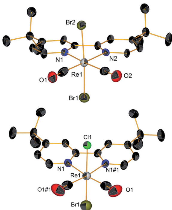
Fig. 1 Crystal structures of compound 1 (top) and the [\text{Re}(\text{CO})_2(\text{Bu}_2\text{bpy})\text{BrCl}] complex (CI-1) obtained from the attempted crystallization of 2 in \text{CHCl}_3 under inert atmosphere. Thermal ellipsoids are at 30% probability.
