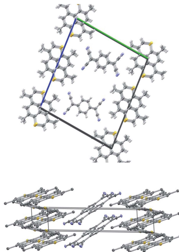
Fig. 4 Crystal packing of TMDTP·TCNQ. Top view approx. along a -axis. Bottom view approx. along c -axis. Thermal ellipsoid probabilities are drawn at 50%. The asymmetric unit comprises half a molecule of TMDTP from each of the two differently inclined stacks and a full TCNQ unit. Hydrogens are omitted for clarity. Color coding: carbon: grey; sulfur: yellow nitrogen: blue.
