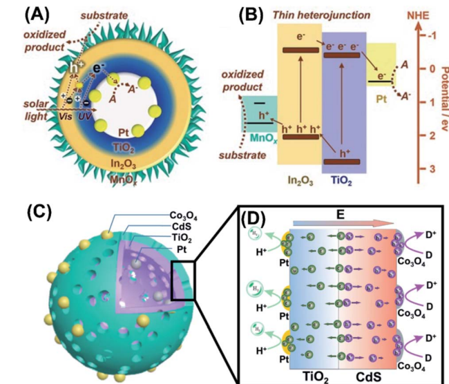
Fig. 17 (A) Microstructural model for \text{TiO}_2/\text{In}_2\text{O}_3 hollow spheres with Pt and \text{MnO}_x respectively deposited at the inner and outer surface. (B) Plausible charge transfer mechanism for superior photocatalytic activity of \text{Pt}/\text{TiO}_2/\text{In}_2\text{O}_3/\text{MnO}_x . Reproduced from ref. 140. Copyright 2016, Wiley. (C) Microstructural model for \text{TiO}_2/\text{CdS} hollow spheres with Pt and \text{Co}_3\text{O}_4 respectively deposited at the inner and outer surface. (D) Plausible charge transfer mechanism for superior photocatalytic activity of \text{Pt}/\text{TiO}_2/\text{In}_2\text{O}_3/\text{Co}_3\text{O}_4 . Reproduced with permission from ref. 136. Copyright 2016, Wiley.
