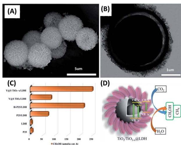
Fig. 8 (A and B) SEM and TEM images of Y@S-TiO 2-x /LDH. (C) Comparative results of CO 2 reduction in terms of CH 3 OH production under visible light illumination. (D) Plausible charge transfer mechanism for superior photocatalytic efficiency of Y@S-TiO 2-x /LDH toward CO 2 reduction. Reproduced with permission from ref. 98. Copyright 2019, American Chemical Society.
