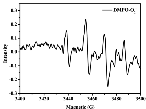
Fig. 5 EPR spectra of DMPO-captured \text{O}_2^{\cdot-} in HBr-photocatalyzed HMF oxidation.
