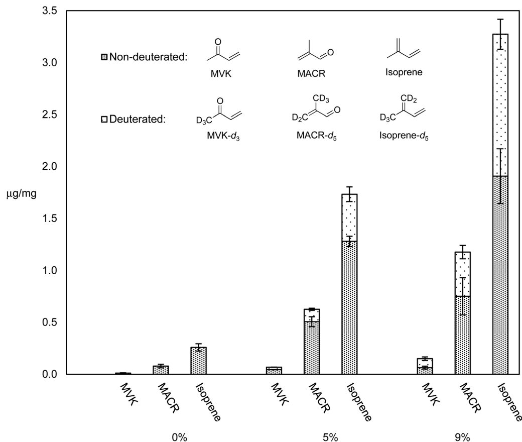
Fig. 4 Comparative levels of major degradation products and their deuterated isotopologues encountered in the aerosol GP from dabbing pure THC (0% β-myrcene-d 6 ), THC with 5% β-myrcene-d 6 , and THC with 9% β-myrcene-d 6 . Error bars are SEM.
