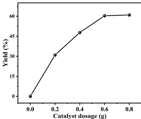
Fig. 6 Effect of catalyst dosage on the decarboxylation of butylene carbonate. Reaction conditions: butylene carbonate (20.0 g), reaction temperature ( 185 \text{ }^\circ\text{C} ), vacuum degree (5 kPa), reaction time (180 min).
