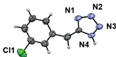
Fig. 5 ORTEP diagram of compound 5k.
