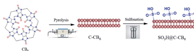
Fig. 2 Preparation of sulfonic acid functionalized nitrogen-rich carbon \text{SO}_3\text{H}@N\text{-C}/\text{CB}_6 .
