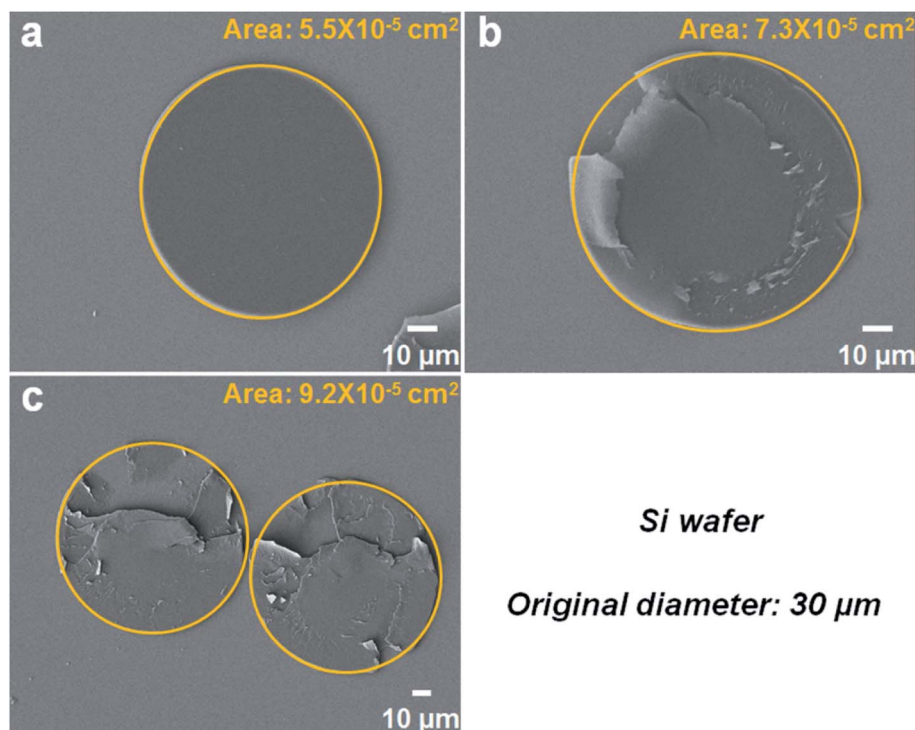
Fig. 3 SEM images of flattened PS particles after deformation at 140 ^{\circ}\text{C} and bonded in the deformed state by cooling below T_g with different adhesive area. (a) Adhesive area: 5.5 \times 10^{-5} \text{ cm}^2 . (b) Adhesive area: 7.3 \times 10^{-5} \text{ cm}^2 . (c) Adhesive area: 9.2 \times 10^{-5} \text{ cm}^2 .
