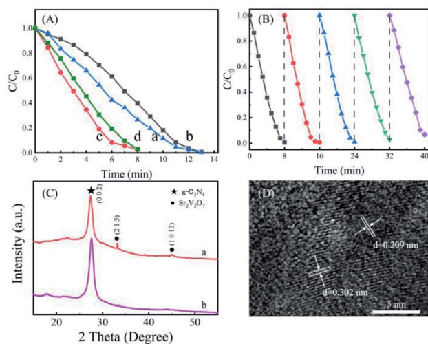
Fig. 4 (A) Time course of C/C_0 of Cr(VI) contained tartaric acid (a) without any photocatalysts, with (b) g\text{-C}_3\text{N}_4 , with (c) g\text{-C}_3\text{N}_4\text{-Sr}_2\text{V}_2\text{O}_7 (0.12 wt%) nanohybrid, and with (d) g\text{-C}_3\text{N}_4\text{-Sr}_2\text{V}_2\text{O}_7 (0.06 wt%) nanohybrid; (B) photocatalytic recycling of the nanohybrid for Cr(VI) reduction; (C) the XRD patterns of the g\text{-C}_3\text{N}_4\text{-Sr}_2\text{V}_2\text{O}_7 nanohybrid before recycling experiment (a) and after recycling experiment (b); (D) HRTEM image of the g\text{-C}_3\text{N}_4\text{-Sr}_2\text{V}_2\text{O}_7 nanohybrid after recycling experiment.
