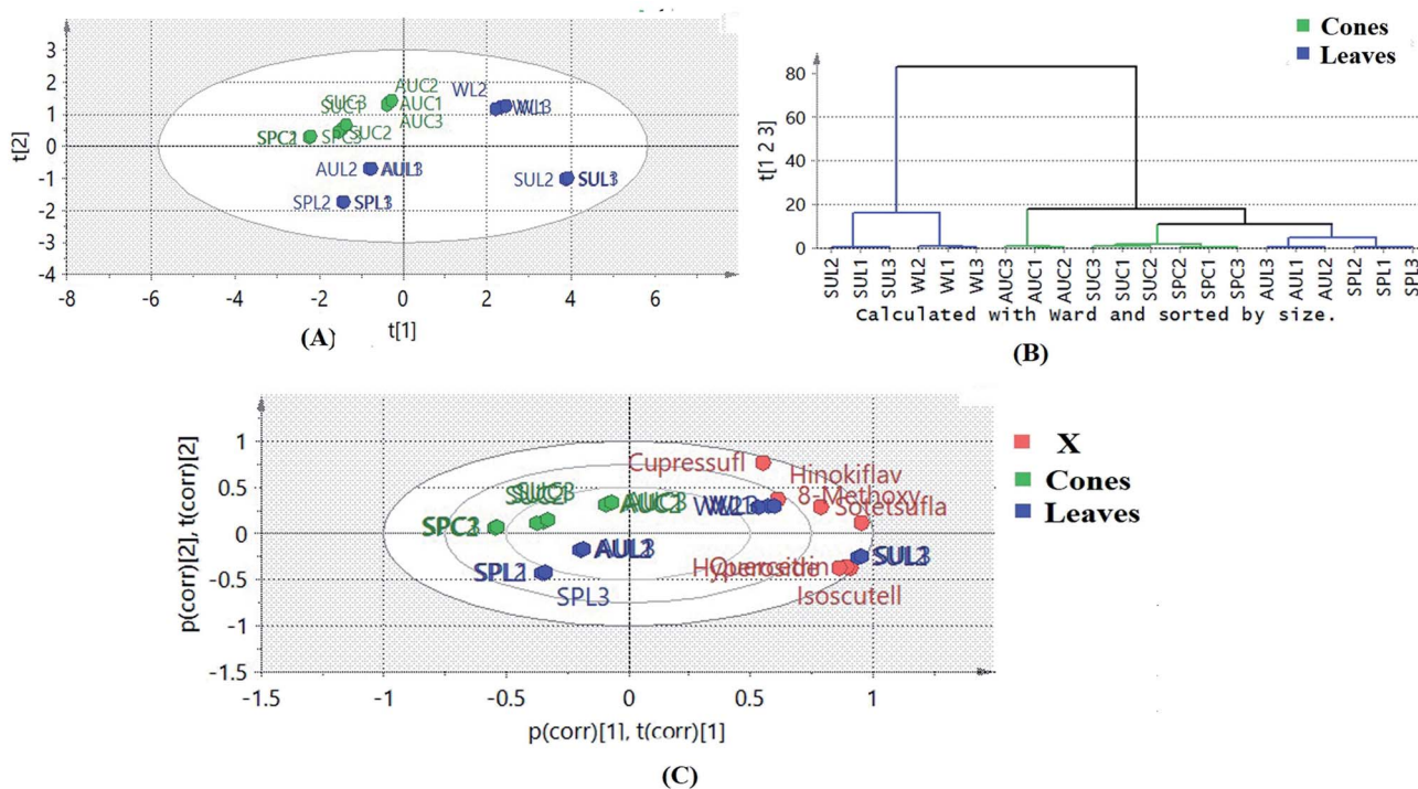
Fig. 5 (A) Biplot (co-chart of scores and loading plots) of different leaf and cone samples of Platykladus and the targeted isolated flavone and biflavone loadings; SPL = spring leaves, SUL = summer leaves, AUL = autumn leaves, WIL = winter leaves, SPC = spring cones, AUC = autumn cones and SUC = summer cones. (B) Dendrogram derived from the hierarchical cluster analysis, based on the Ward method, of the different leaf and cone samples of Platykladus .
