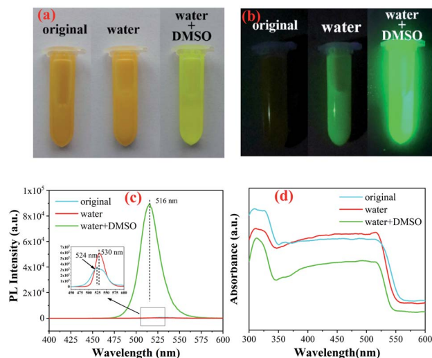
Fig. 1 The digital optical photos of \text{Cs}_4\text{PbBr}_6 samples of original, water and water + DMSO under ambient light (a) and under UV lamp (b); the photoluminescence emission (c) and absorbance spectrum (d).
