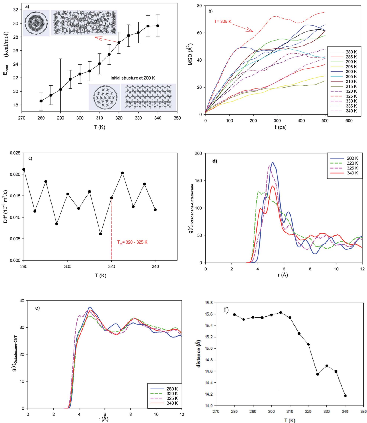
Fig. 1 Normal system consisting of 17 octadecane molecules in the capped (25,0) CNT with a length of 42.68 \text{\AA} . (a) Configurational energy, (b) mean square displacement (MSD), (c) self-diffusion coefficient, (d) octadecane–octadecane radial distribution function (RDF), (e) octadecane–CNT RDF, and (f) average end-to-end distance.
