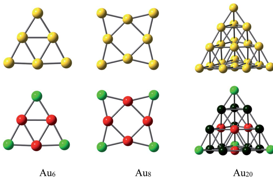
Fig. 3 Equilibrium geometries and NBO charges of Au N clusters considered ( N = 6, 8, 20 ). Color range in a.u.: green, more positive than 0.07; red, more negative than -0.07 ; black, less positive than 0.02.
