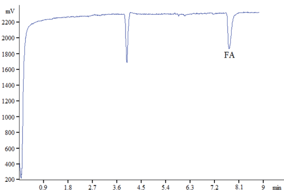
Fig. 3 Electropherogram of substance to be tested. (Condition: 65 cm \times 50 \mu\text{m} i.d. fused silica; applied voltage: 18 kV; injection time: 15 s; C_{\text{Ag(III)}} = 5.0 \times 10^{-5} mol \text{L}^{-1} in 0.01 mol \text{L}^{-1} NaOH; C_{\text{luminol}} = 2 mmol \text{L}^{-1} in 5 mmol \text{L}^{-1} sodium tetraborate; FA: 100 mg \text{L}^{-1} ).
