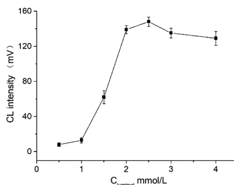
Fig. 4 Effect of the concentration of luminol on CL intensity. (Condition: 65 cm \times 50 \mu\text{m} i.d. fused silica; applied voltage: 18 kV; injection time: 15 s; C_{\text{Ag(III)}} = 5.0 \times 10^{-5} mol \text{L}^{-1} in 0.03 mol \text{L}^{-1} NaOH; luminol in 5 mmol \text{L}^{-1} sodium tetraborate; FA: 100 mg \text{L}^{-1} ).
