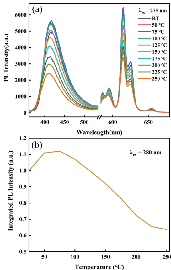
Fig. 13 (a) Temperature-dependent PL spectra and (b) integrated intensity-temperature curve of R800, \lambda_{\text{ex}} = 275 \text{ nm} .
