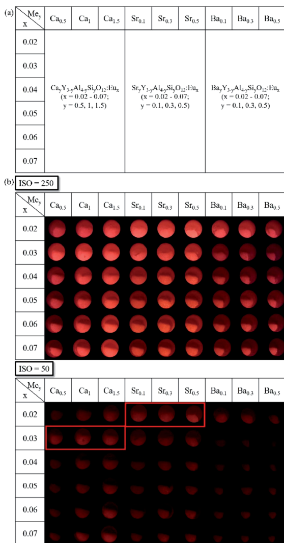
Fig. 3 (a) Designed composition map for further screening and (b) fluorescence images of the \text{Me}_x\text{Y}_{3-y}\text{Al}_{5-y}\text{Si}_y\text{O}_{12}:\text{Eu}_x ( \text{Me} = \text{Ca}, \text{Sr}, \text{Ba} ; x = 0.02-0.07 , y = 0.1-1.5 ) library under 254 nm excitation, the library was calcined at 1300 °C for 2 h in an air atmosphere.
