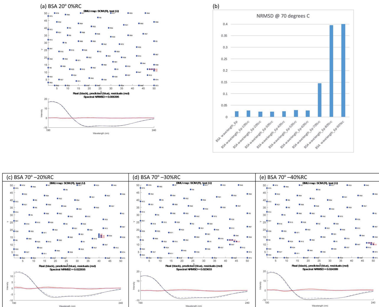
Fig. 2 SOMSpec output for BSA (a) at 20 °C with 0% RC. (b) SOMSpec spectral NRMDSs for 70 °C BSA with different degrees of randomisation and output for 70 °C with (c) -20% RC, (d) -30% RC, and (e) -40% RC. The x and y axis labels indicate the self-organising map size and node positions for each run.
