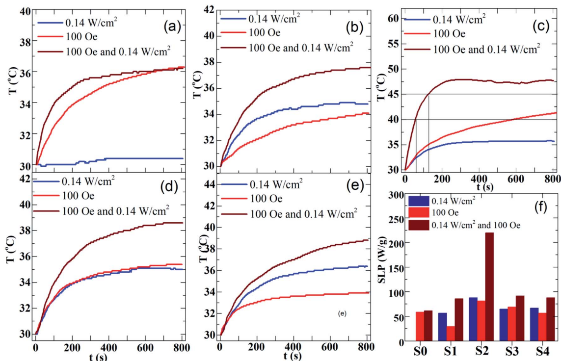
Fig. 9 Photothermal heating and magnetic inductive heating curves of the \text{MnFe}_2\text{O}_4 -Ag hybrid nanoparticles suspension ( 2 \text{ mg mL}^{-1} ): (a) S0 sample, (b) S1 sample, (c) S2 sample, (d) S3 sample and (e) S4 sample. (f) The field-dependent SAR values of the \text{MnFe}_2\text{O}_4 -Ag hybrid nanoparticles suspension.
