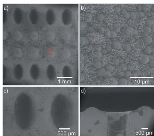
Fig. 5 The SEM images of the bio-fabricated membrane. (a) The surface is composed by elliptic micro-stomata array and micro-papillae array. (b) The papilla surface is covered by micro sphere and ZnO nano-rod. The diameter and height of nano-rods are 90–110 nm and 2 \mu\text{m} , respectively. (c and d) The top view and side view of the elliptic stomata.
