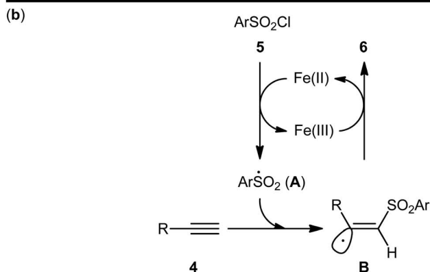
Scheme 2 (a) Fe-catalyzed chlorosulfonylation of terminal alkynes 4 with arylsulfonyl chlorides 5 ; (b) proposed mechanism for the formation of ( Z )- \beta -chlorovinyl sulfones 6 .
