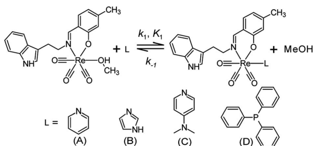
Fig. 4 Schematic diagram for the substitution of methanol by various neutral mono-dentate ligands (A) pyridine, (B) imidazole, (C) 4-dimethylaminopyridine and (D) triphenylphosphine in the \text{fac}[\text{Re}(\text{CO})_3(5\text{Me-Sal-Trypt})(\text{MeOH})] (2) complex.
