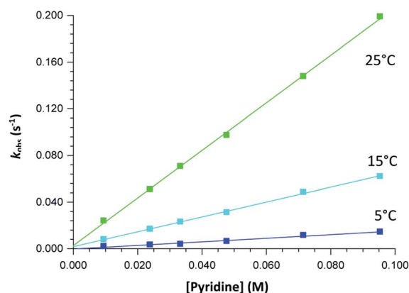
Fig. 5 Plot of k_{\text{obs}} versus [pyridine] for the reaction between \text{fac}[\text{Re}(\text{CO})_3(5\text{Me-Sal-Trypt})(\text{MeOH})] (2) and pyridine at a range of temperatures with [\text{Re complex}] = 4 \times 10^{-4} \text{ M} and [\text{pyridine}] = 0.010 \text{ M} - 0.095 \text{ M} collected in methanol at 380 nm, yielding linear relationships.
